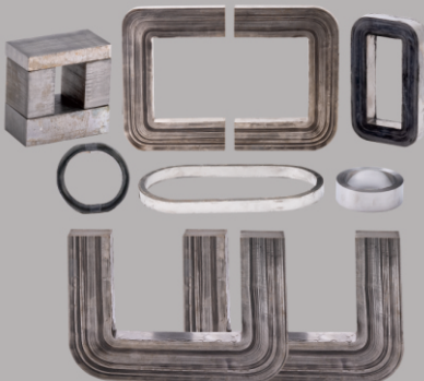
Nano Crystalline Cut Core and Blocks
