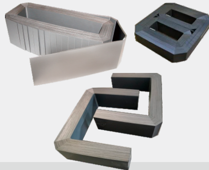
Distributed Gap cores & Butt Cores
