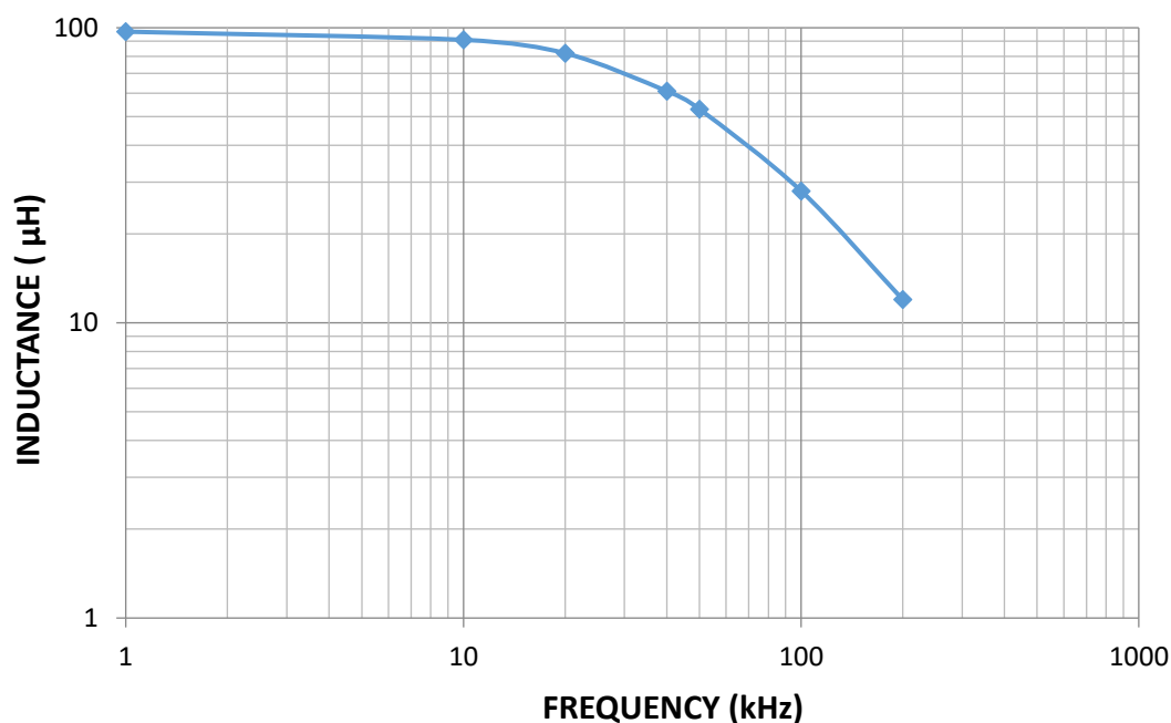
TYPICAL CURVE OF INDUCTANCE VS FREQUENCY
