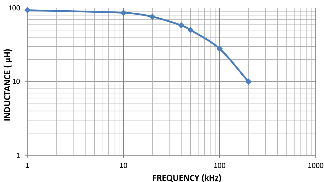
TYPICAL CURVE OF INDUCTANCE VS FREQUENCY
